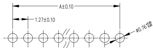
PCB LAYOUT
