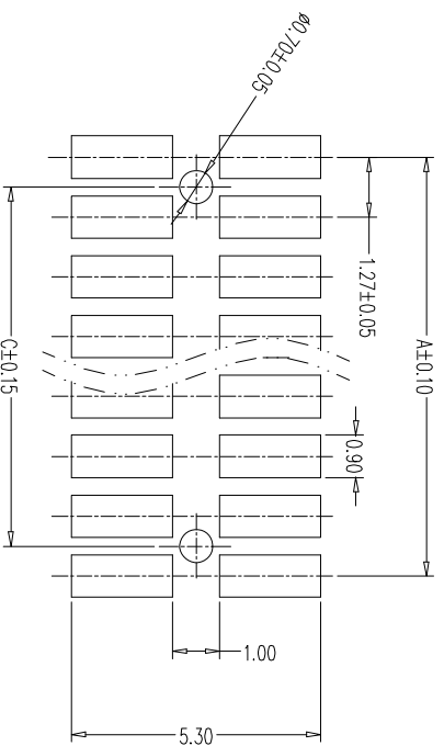
PCB LAYOUT
