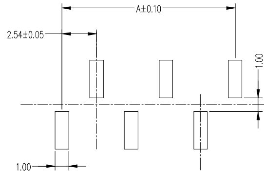
B TYPE Recommended P.C.B Layout
