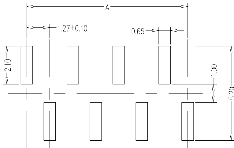
A type Recommended P.C.B Layout
